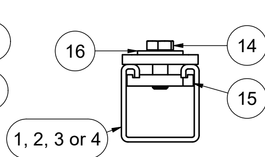
Standard mounting sliding nut (1 : 2)
