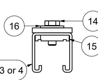
Mounting closed side (1 : 2)
